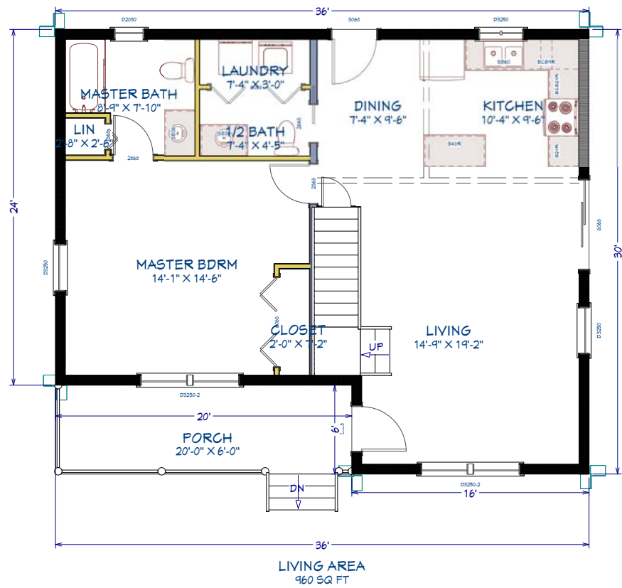
1st Floor
